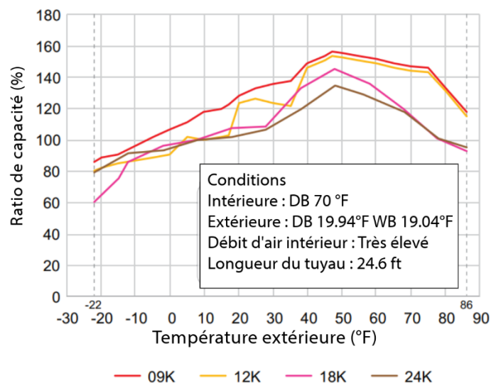
Chauffage
